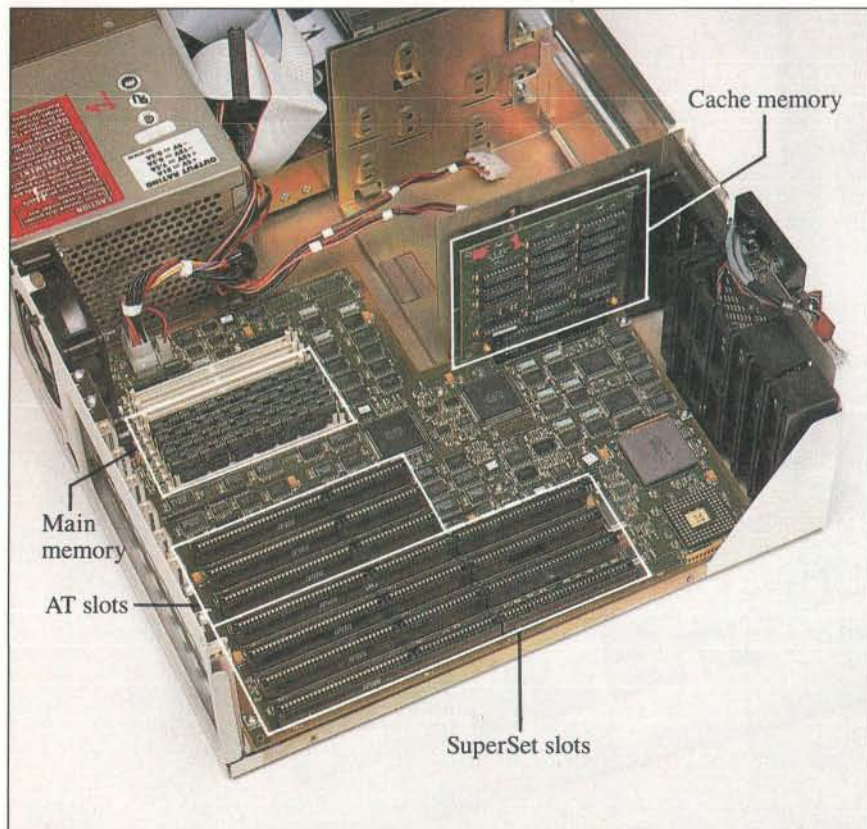
Photo 1: The Z-386/33 motherboard. SIMM-mounted system RAM and a half-length cache board make memory upgrades a snap.
